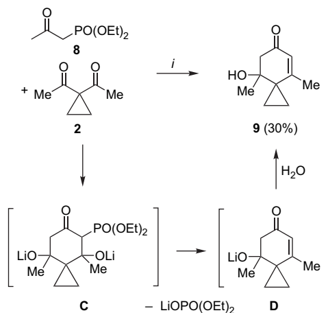
Scheme 4. Synthesis of spirocyclopropane 9 , (i): (1) LDA (2.0 equiv), 8 (1.0 equiv), THF, 1 h, 0 °C; (2) 2 (1.0 equiv), -78 \rightarrow 20 °C, 14 h.
