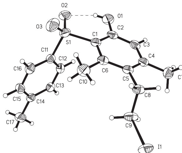
Figure 2. Ortep plot of 4f .
