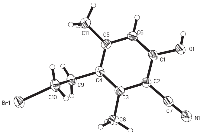
Figure 3. Ortep plot of 7b .
