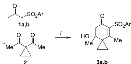
Scheme 1. Synthesis of 3a,b , (i): (1) LDA (2.0 equiv), 1a,b (1.0 equiv), THF, 1 h 0 °C; (2) 2 (1.0 equiv), -78 \rightarrow 20 °C, 14 h.
