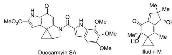
Chart 1. Natural cancerostatic spirocyclopropanes.
