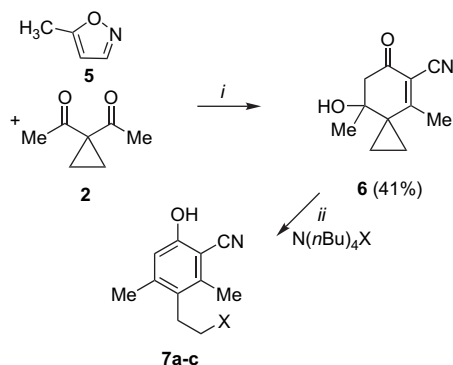
Scheme 3. Synthesis of 7a–c , (i): (1) LDA (2.0 equiv), 5 (1.0 equiv), THF, 1 h, 0 °C; (2) 2 (1.0 equiv), -78 \rightarrow 20 °C, 14 h; (ii): n\text{-Bu}_4\text{NX} (1.0 equiv), \text{BF}_3 \cdot \text{OEt}_2 (0.5 equiv), -78 \rightarrow 20 °C, 12 h.
