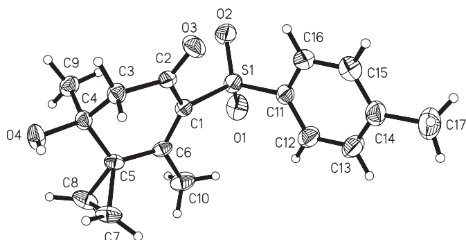
Figure 1. Ortep plot of 3b .
