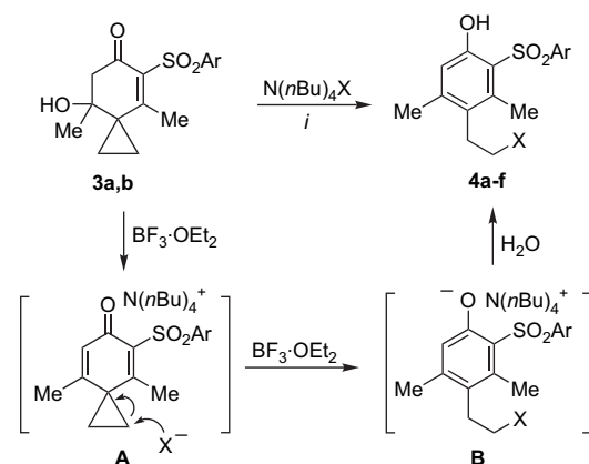
Scheme 2. Synthesis of 4a–f , (i): \text{BF}_3 \cdot \text{OEt}_2 , \text{CH}_2\text{Cl}_2 , -78 \rightarrow 20 °C, 6 h, then 20 °C, 6 h.
