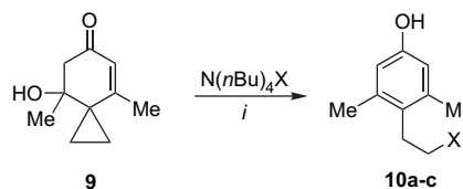
Scheme 5. Reaction of 9 with n\text{-Bu}_4\text{NX} , (i): n\text{-Bu}_4\text{NX} (1.0 equiv), \text{BF}_3 \cdot \text{OEt}_2 (0.5 equiv), -78 \rightarrow 20 °C, 12 h.
